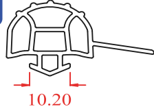
Buzhane kapı fitili. Ice House doors wick.
