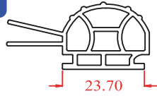
Buzhane kapı fitili. Ice Hosue doors wick.
