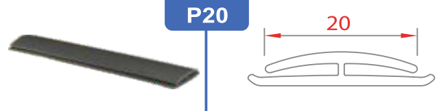
Sanayi tipi buzdolabı yan blok fitili Industrial type Refrigerator side block wicks
